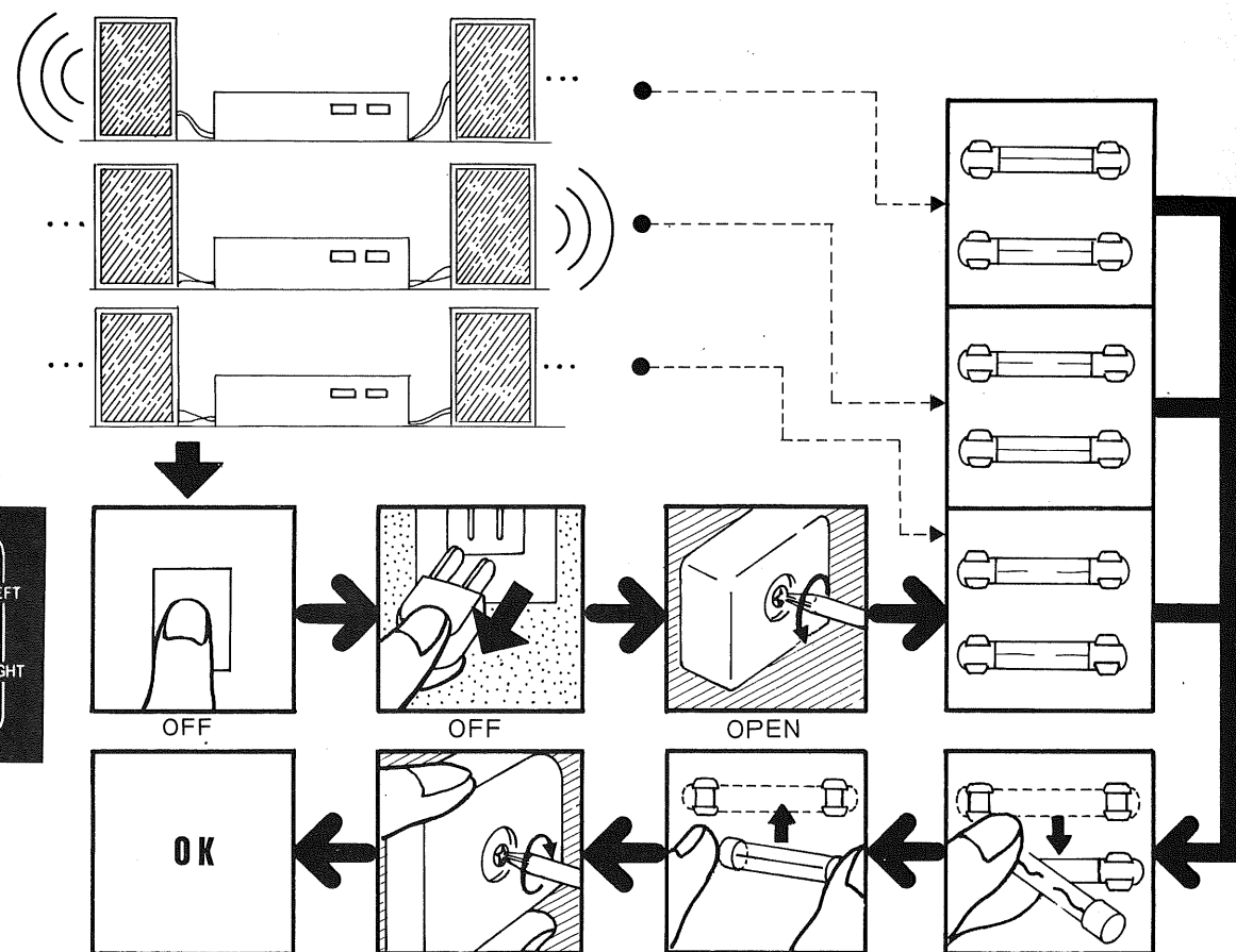
SPEAKER FUSE
